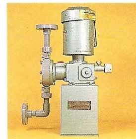
● Union type
